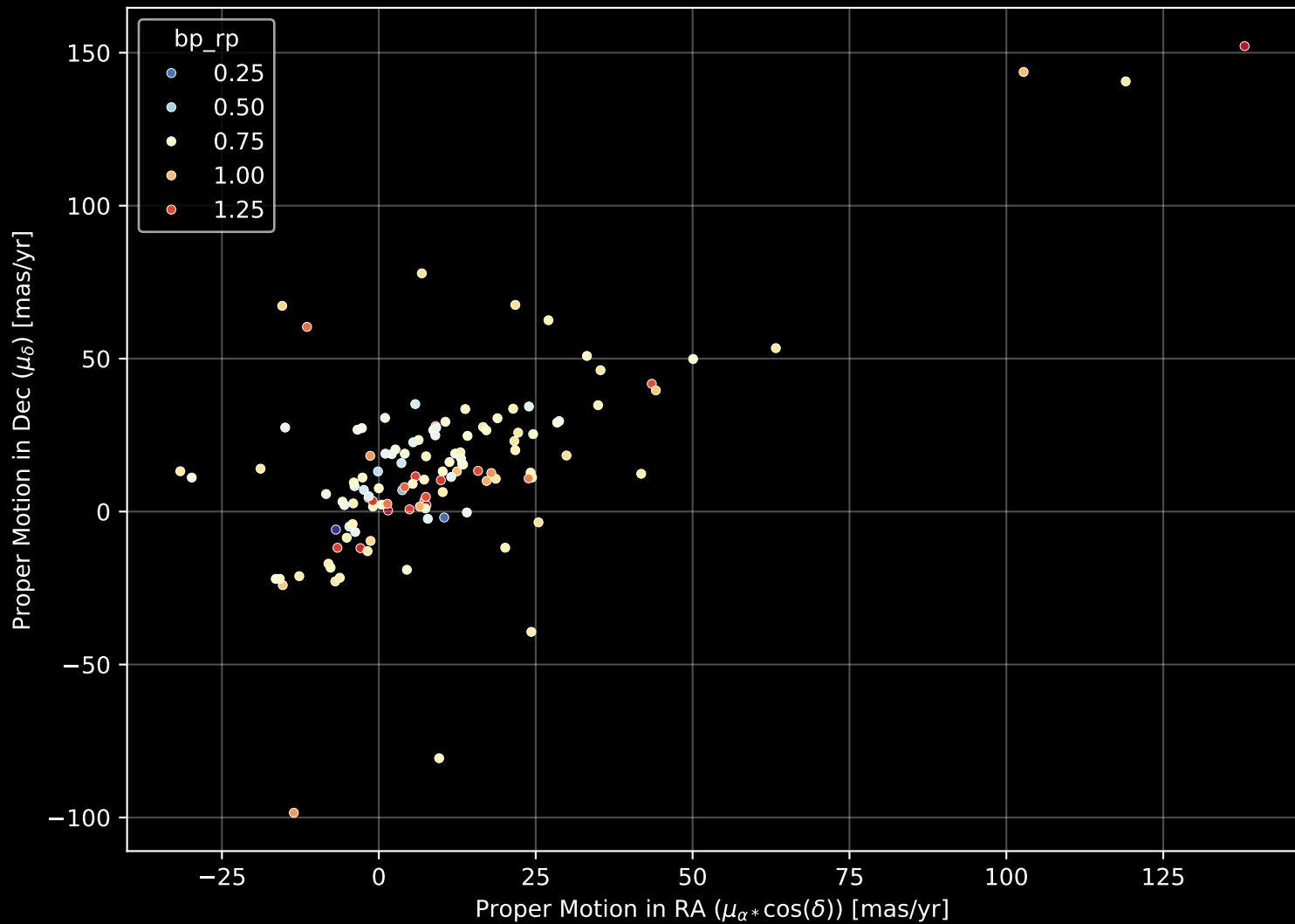
GALAH DR4 Field: [7208] Proper Motion Diagram (n= 124)
