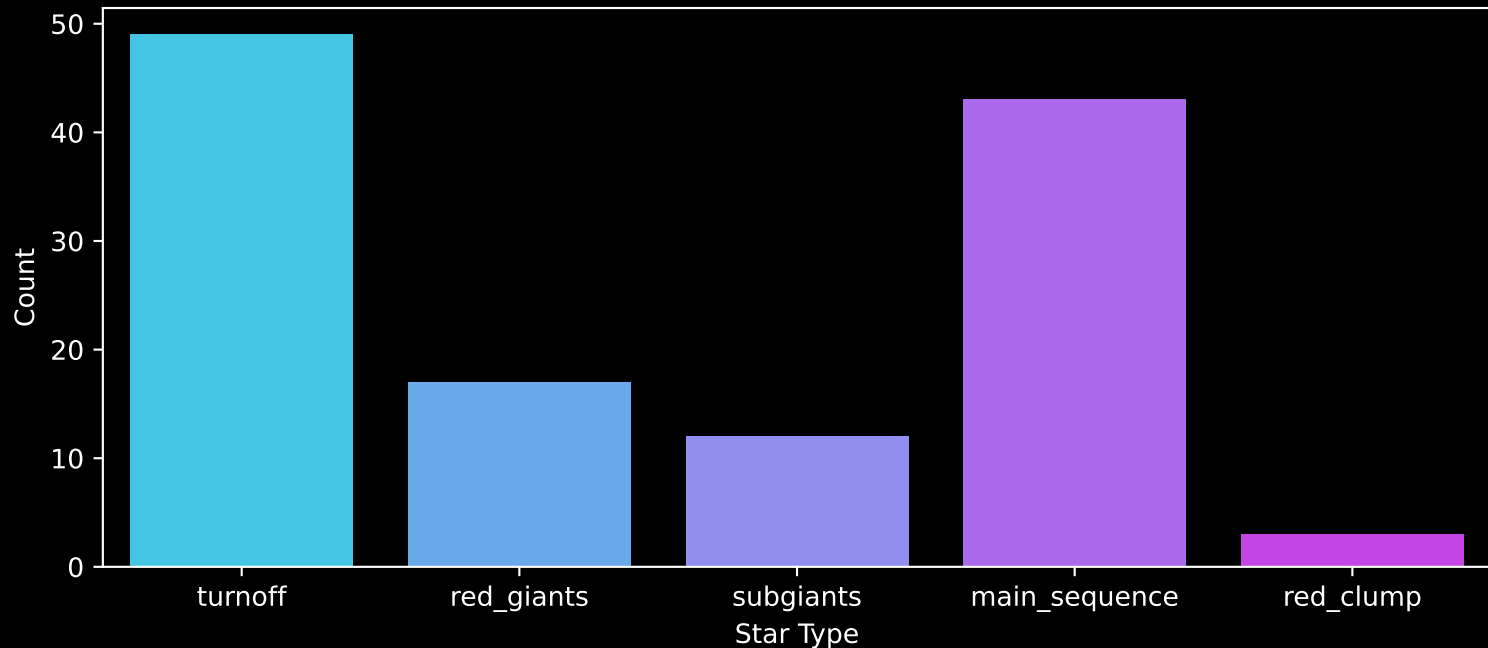
GALAH DR4 Field: [7208] Count plot of Star Type
