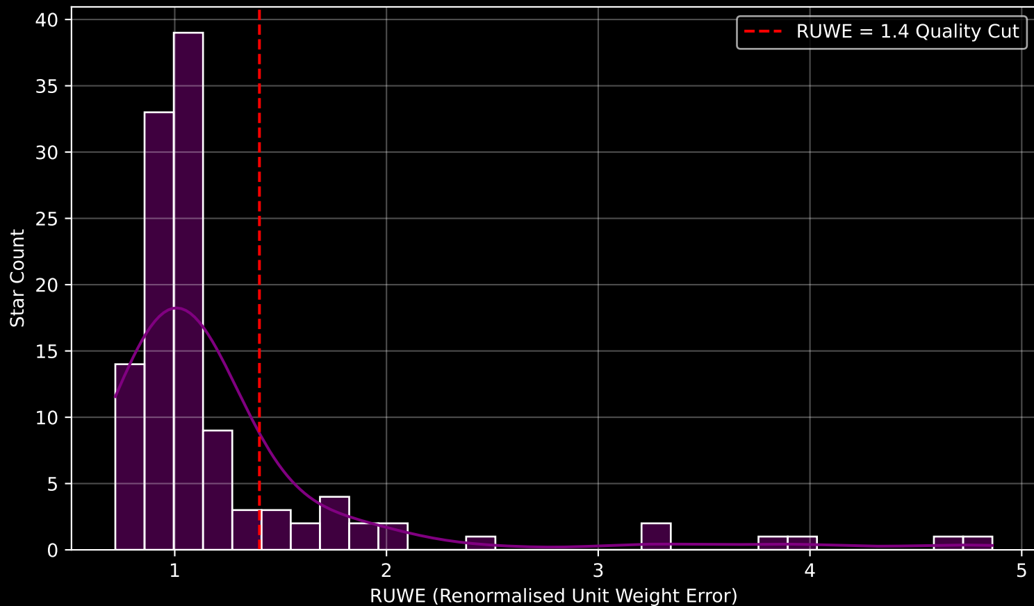
GALAH DR4 Field [7208] RUWE Distribution (n= 118)
